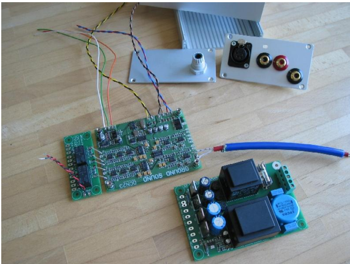
The blue input cable is the top-end NF interconnect cable with mica insulation. The case is a very compact slide-in case for Euro-format boards.
